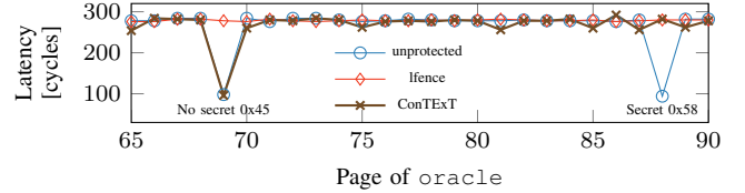
Fig. 3: Evaluation of Figure 1. The unprotected code snippet leaks the secret 'X' (0x58) and public value 'E' (0x45) to the cache (Lines 7 to 8). State-of-the-art lfence-based mitigation (lfence in Line 6) prevents both indices from being cached. A ConTE X T-light annotation (Line 3) prevents the secret index from being cached but allows the public index to be cached, warming up the cache.
