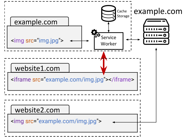
Fig. 3. Example site with a SW implementing a FetchEvent listener, which operates as a network proxy. A third-party ( website1 ) includes an iframe that activates and uses example.com 's SW for fetching the resource.
